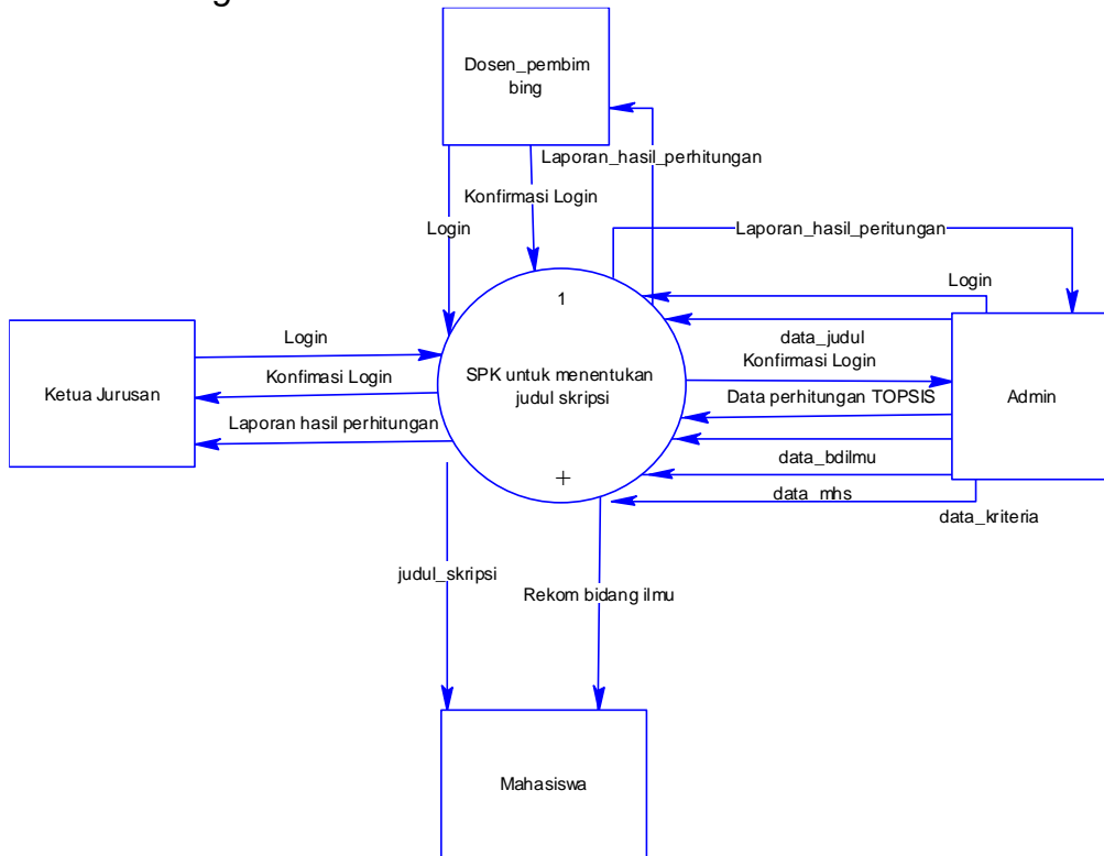
Gambar 2 DFD Level 0
